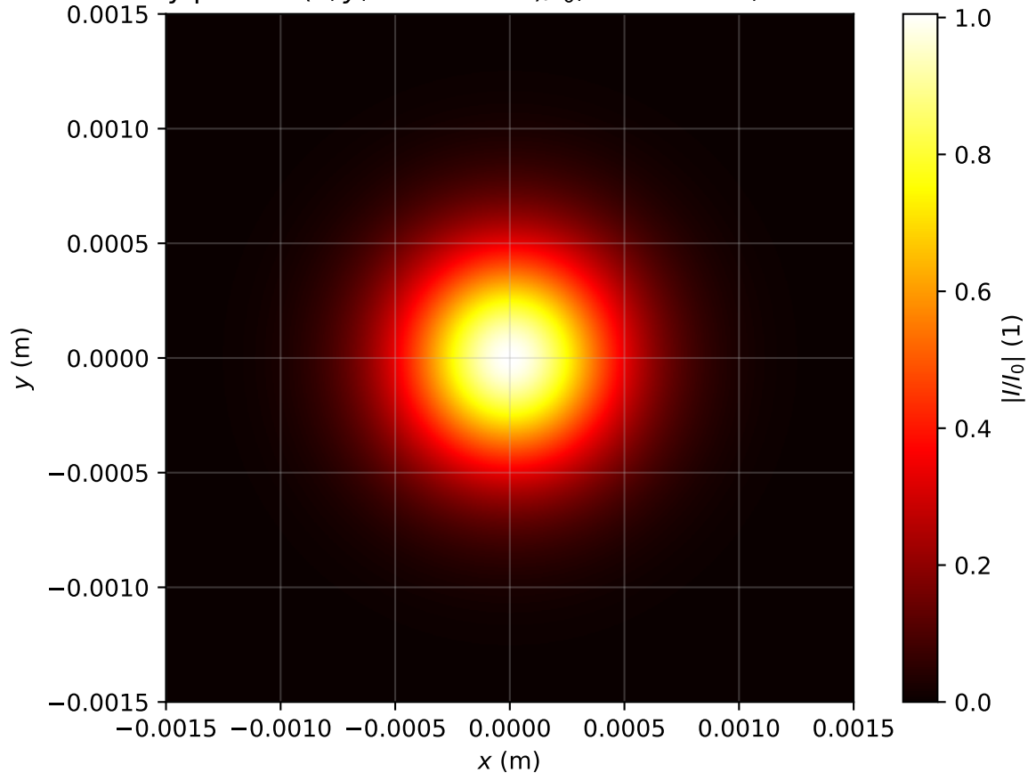
Intensity profile I(x, y, z = 0.876m)/I_0 , Pin=0.4Pcr, artificial time
